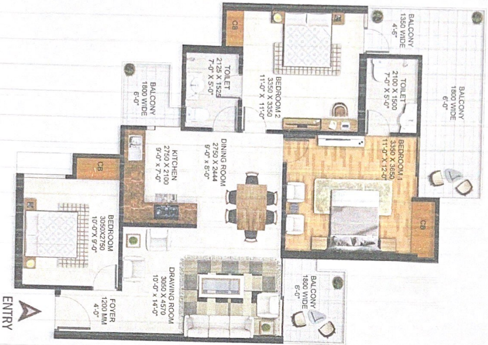
3 BEDROOM + LIVING / DINING + KITCHEN + 2 TOILET + 3 BALCONY
