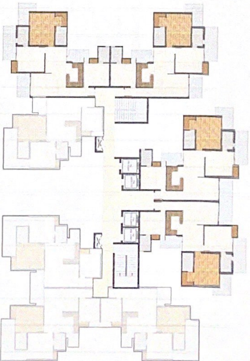
CLUSTER PLAN 3 BHK UNIT (4 No.)
