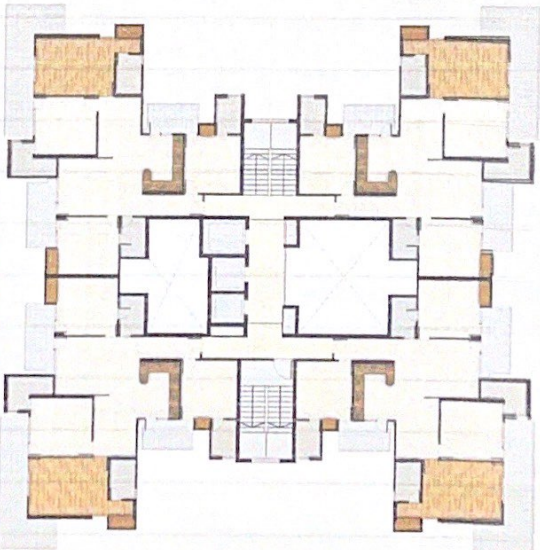
CLUSTER PLAN 4 BHK UNIT (4 No.)
